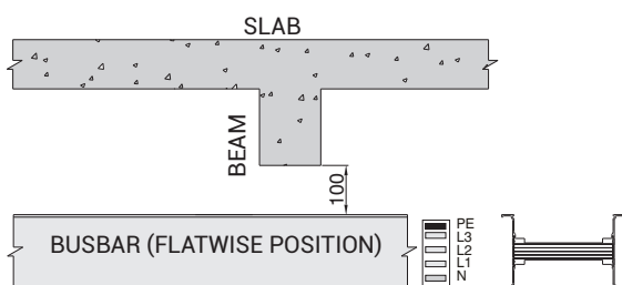
FIGURE-4 CROSSING UNDER A BEAM HORIZONTAL POSITION
