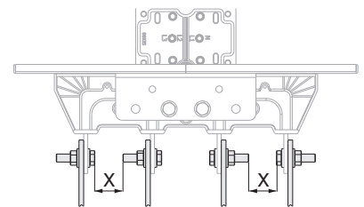
Sample Connection
